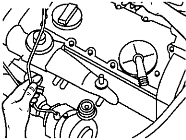
Fit Oil Feed Line
