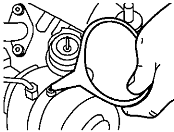
Fill Turbocharger with Oil
