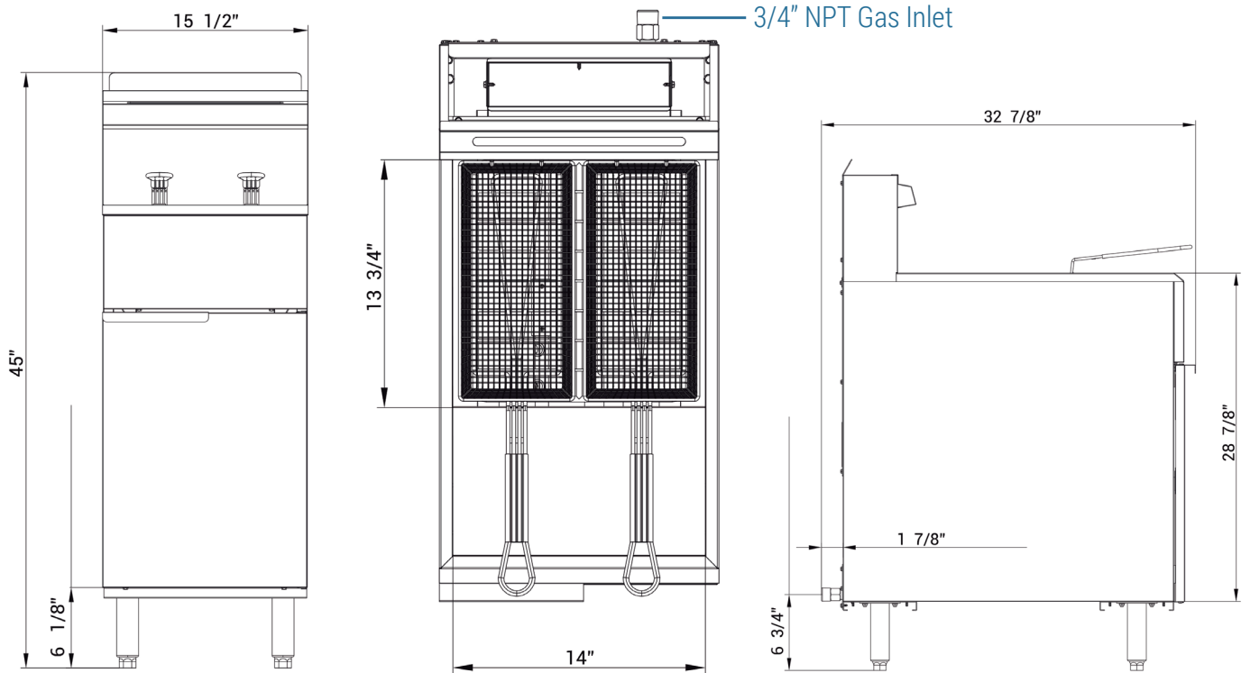
Front View
