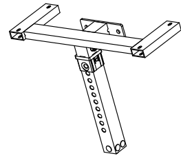
K [1PCS]
