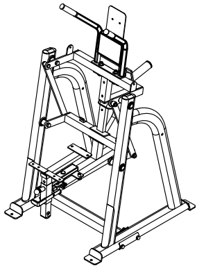
Above shows STEP 3 assembled and completed
