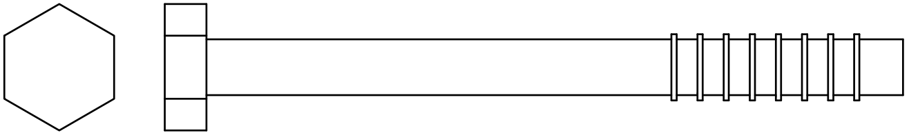
(A1)HEX BOLT 1/2"x3-1/4"L PARTIAL THREAD QTY.2
