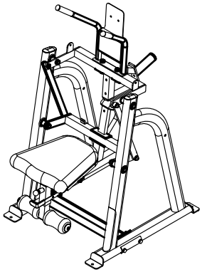
Above shows STEP 4 assembled and completed
