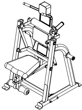
Above shows STEP 6 assembled and completed
