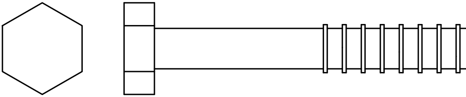
(A1)HEX BOLT 1/2"x3-1/4"L PARTIAL THREAD QTY.2
