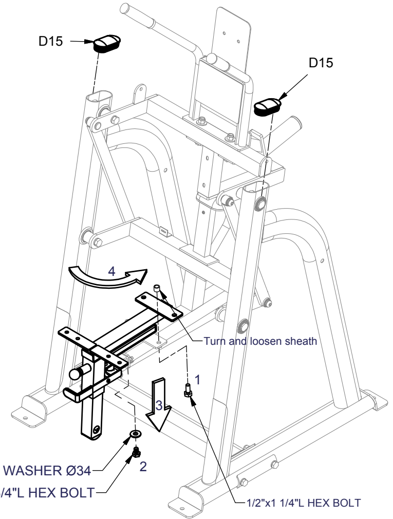
STEP: 1→2→3→4→1→2 tighten all screws as Figure 2 #2→#1
