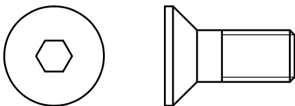
(A6)Co.Noid HEAD BOLT M10X25L PARTIAL THREAD QTY.2
