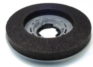
Carborundum \varnothing 410mm Ideal disc for aggressive sanding on cement screeds, removes creases, excess thicknesses and old glues.
