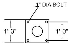
4 BOLT BASE BOLT PATTERN 7/8" BASE PLATE THICKNESS AT ANCHOR BOLT VIEW A-A NOT TO SCALE
