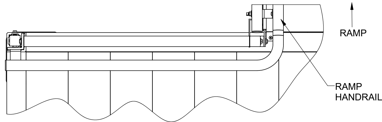
1 2 PLATFORM HANDRAIL TERMINATION DETAIL SCALE 1:4
