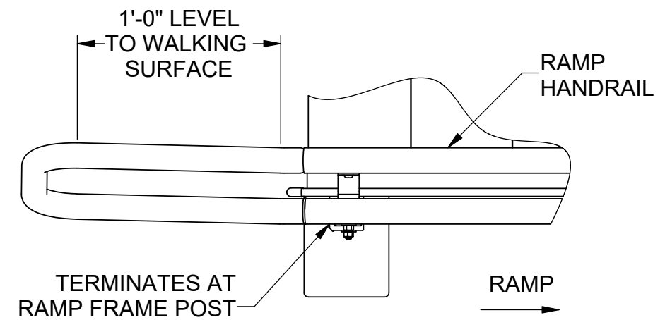
2 2 UPPER/LOWER HANDRAIL LOOP DETAIL SCALE 1:4
