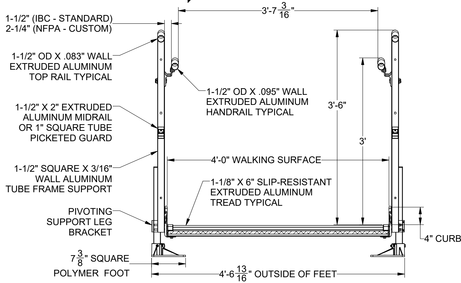
A RAMP CROSS SECTION SCALE 1:6
