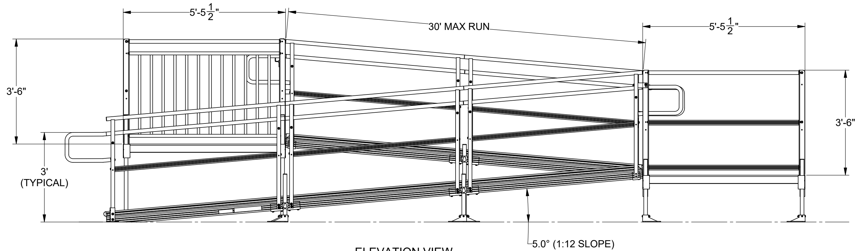
ELEVATION VIEW PATHWAY HD MODULAR ACCESS SYSTEM TWO-LINE RAIL OPTION (GUARDS REQUIRED AT 30" HEIGHT)
