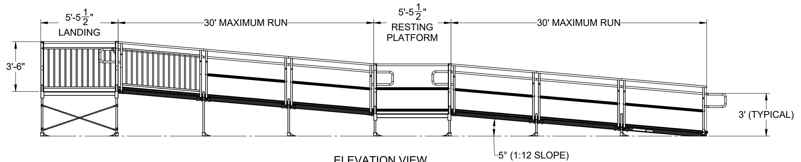
ELEVATION VIEW PATHWAY HD MODULAR ACCESS SYSTEM TWO-LINE RAIL OPTION (GUARDS REQUIRED AT 30" HEIGHT)
