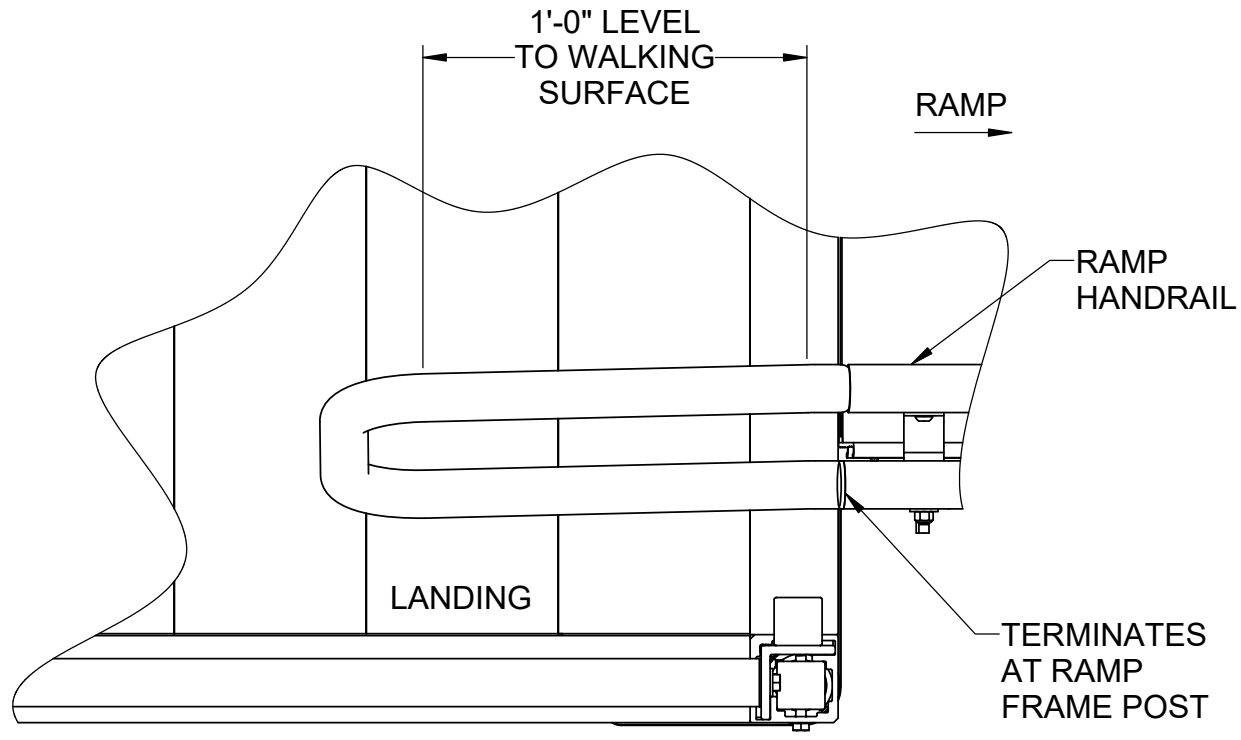
2 UPPER/LOWER HANDRAIL LOOP DETAIL 2 SCALE 1:3
