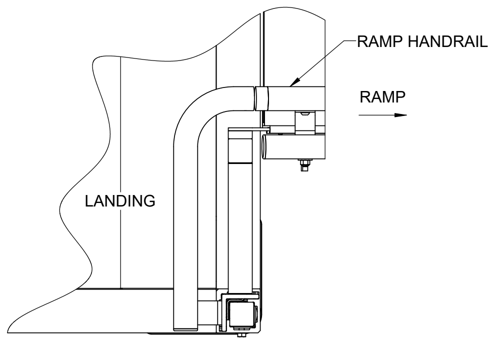
1 PLATFORM HANDRAIL TERMINATION DETAIL 2 SCALE 1:3
