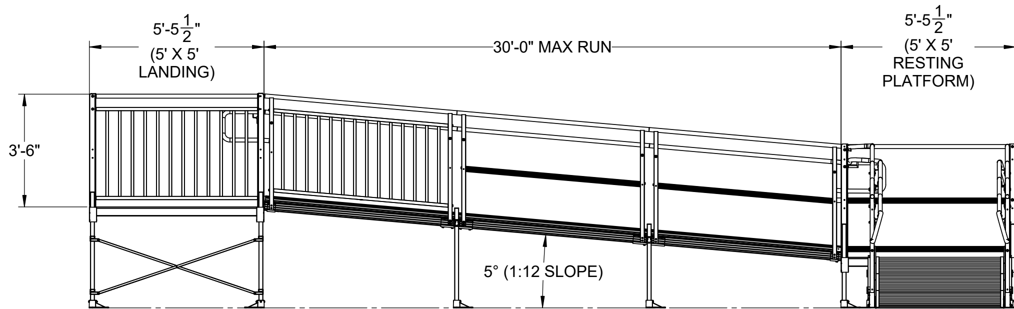
ELEVATION VIEW PATHWAY HD MODULAR ACCESS SYSTEM TWO-LINE RAIL OPTION (GUARDS REQUIRED AT 30" HEIGHT)
