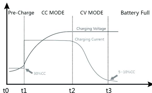
Figure 2. Charging characteristic curve.
