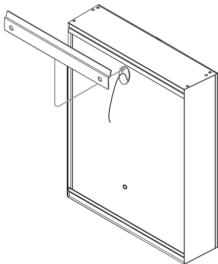
Fig. 3. - Mounting Point
