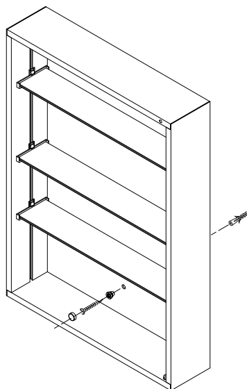
Fig. 4. - Internal fixing point
