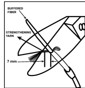
TRIM ARAMID STRENGTH MEMBERS BACK TO CABLE JACKET
