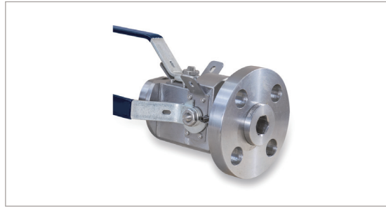
■ Floating Split Body ■ Ball Valves
