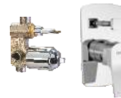
High flow single lever concealed diverter Exposed part F1021721 ₹ 2,900 Concealed part F4030101 ₹ 4,320 Set ₹ 7,220
