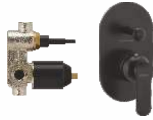
High flow single lever concealed diverter Exposed part F1018721BM ₹ 5,390 Concealed part F4030101BM ₹ 5,620 Set ₹ 11,010
