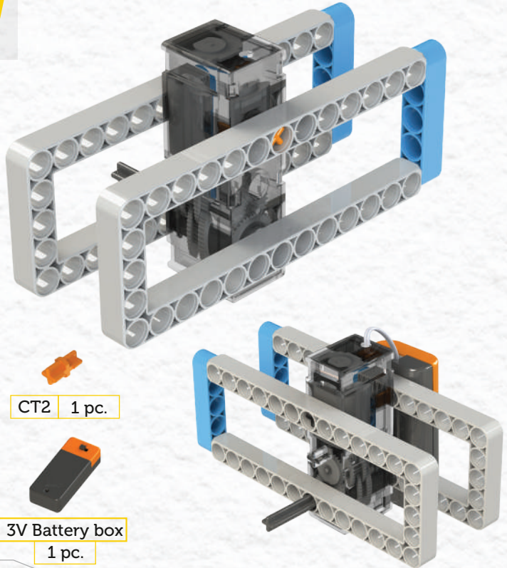
Backside View
