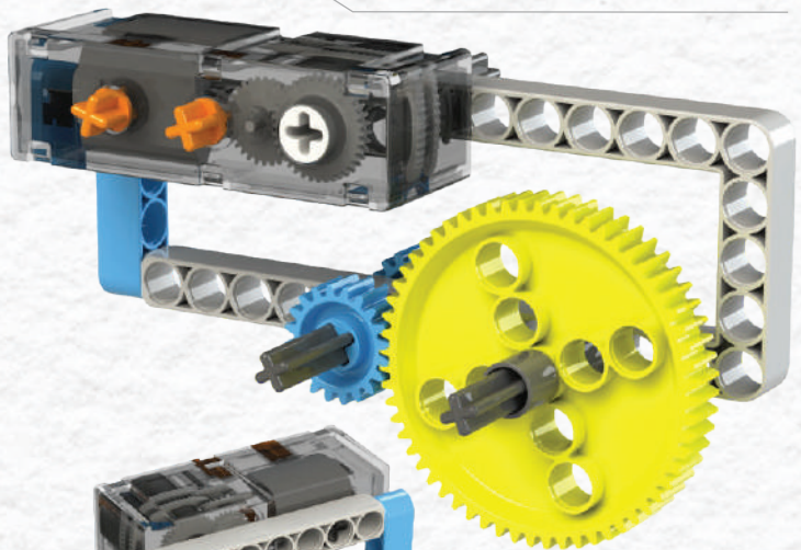
Backside View
