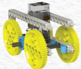
Backside View
