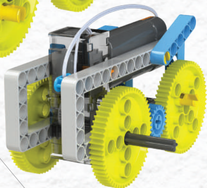
Backside View
