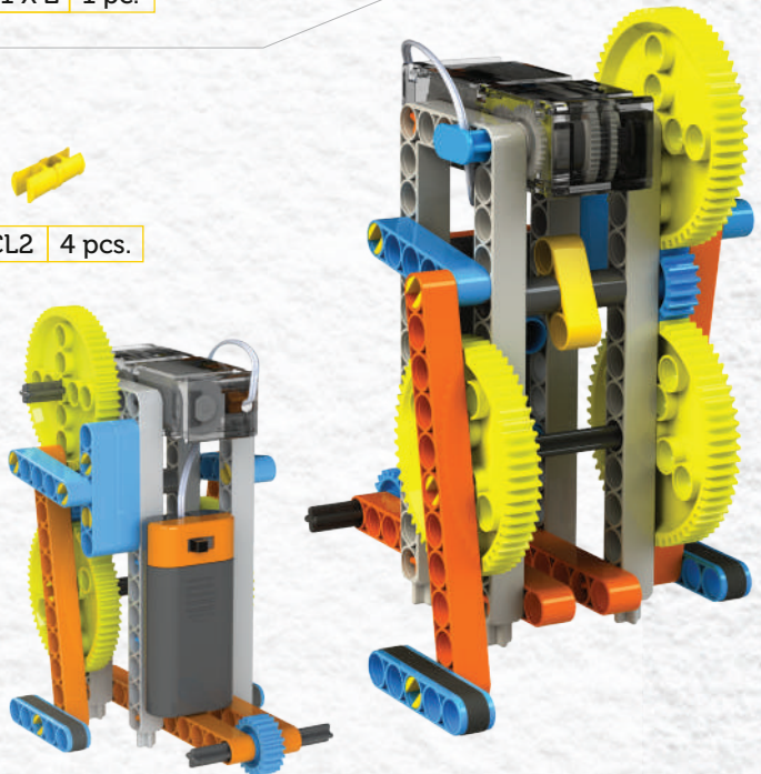
Backside View
