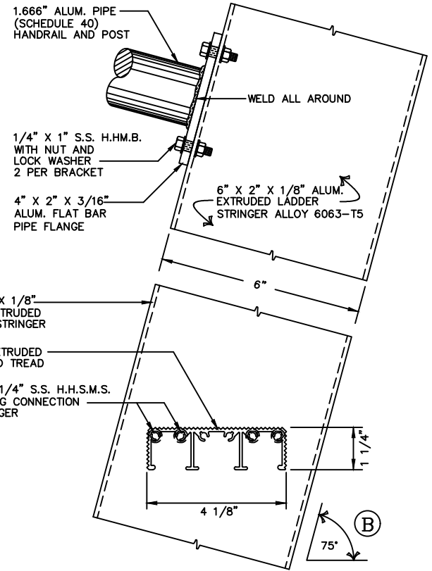
(1) TREAD DETAIL 3" = 1' - 0"
