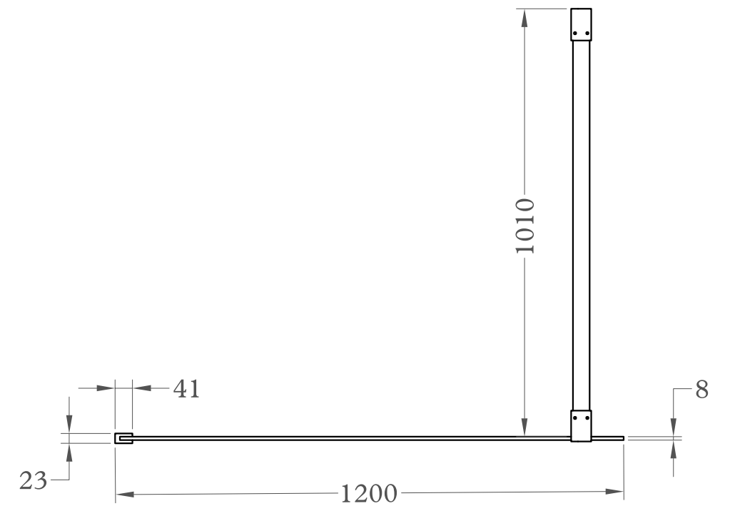
Top View
