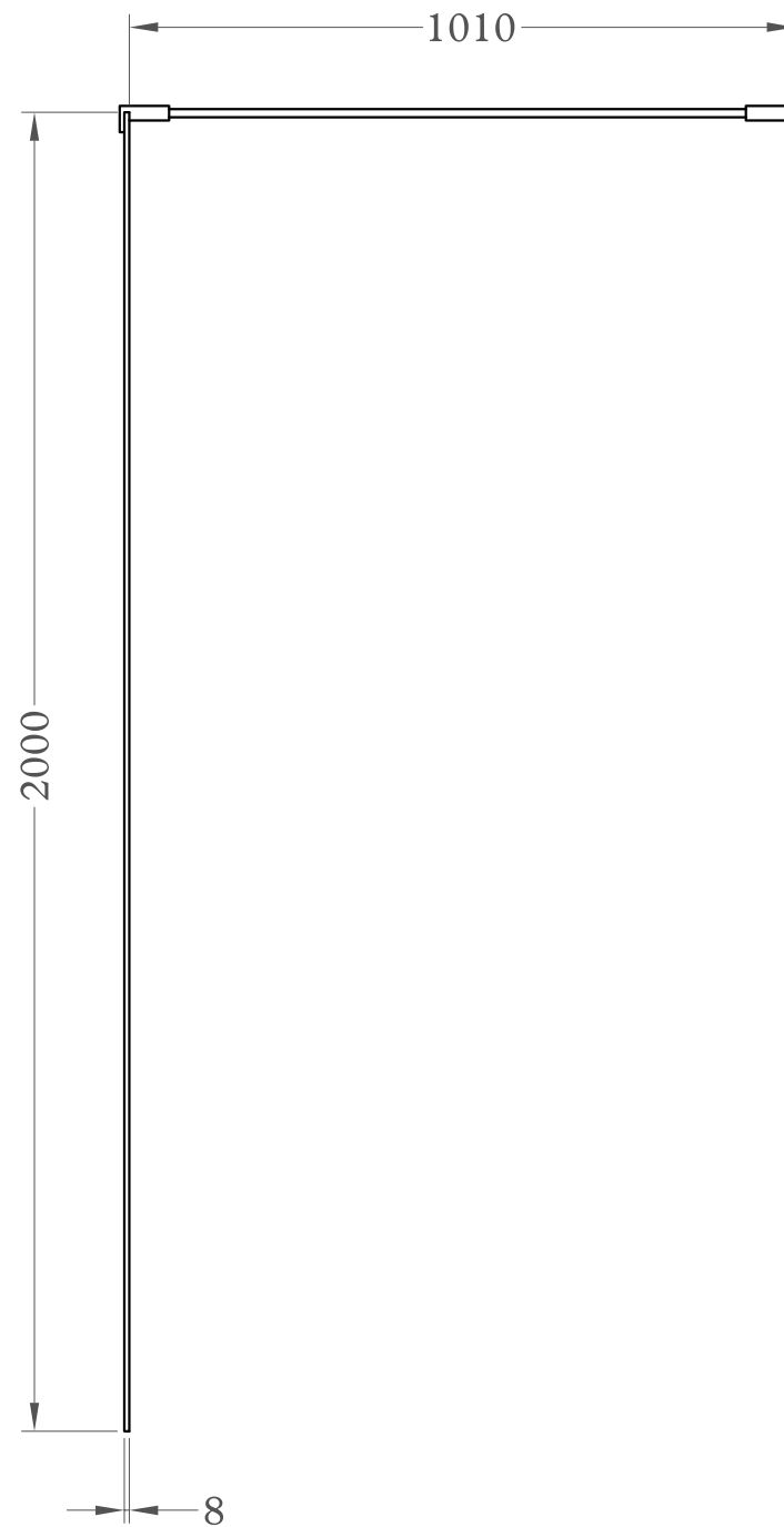
Side View
