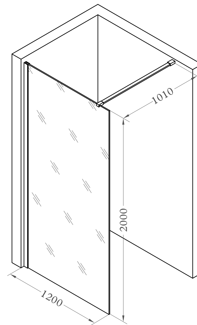
Isometric View
