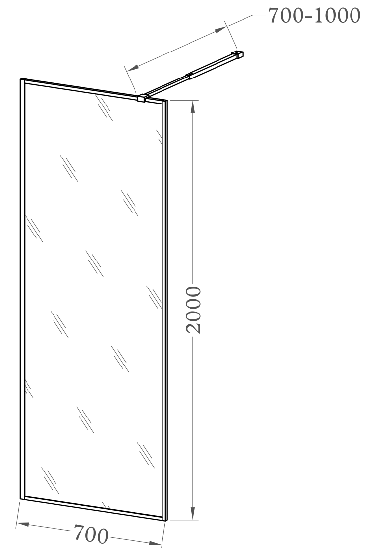
Isometric View
