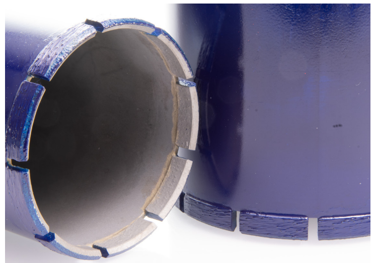
C-43 Asphalt & Prestressed 1-1/4"-7 thread .315" Segments
