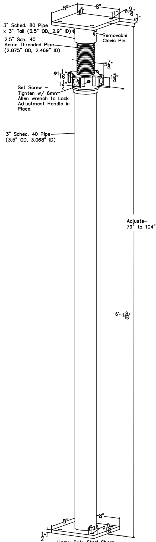
Heavy Duty Steel Shore STL-79HD Adjusts 25" (79" to 104") Tighten Set Screw w/ 6mm Allen Wrench to Lock Handle in place. 30,000 Lb. Load Capacity 83 Lbs.
