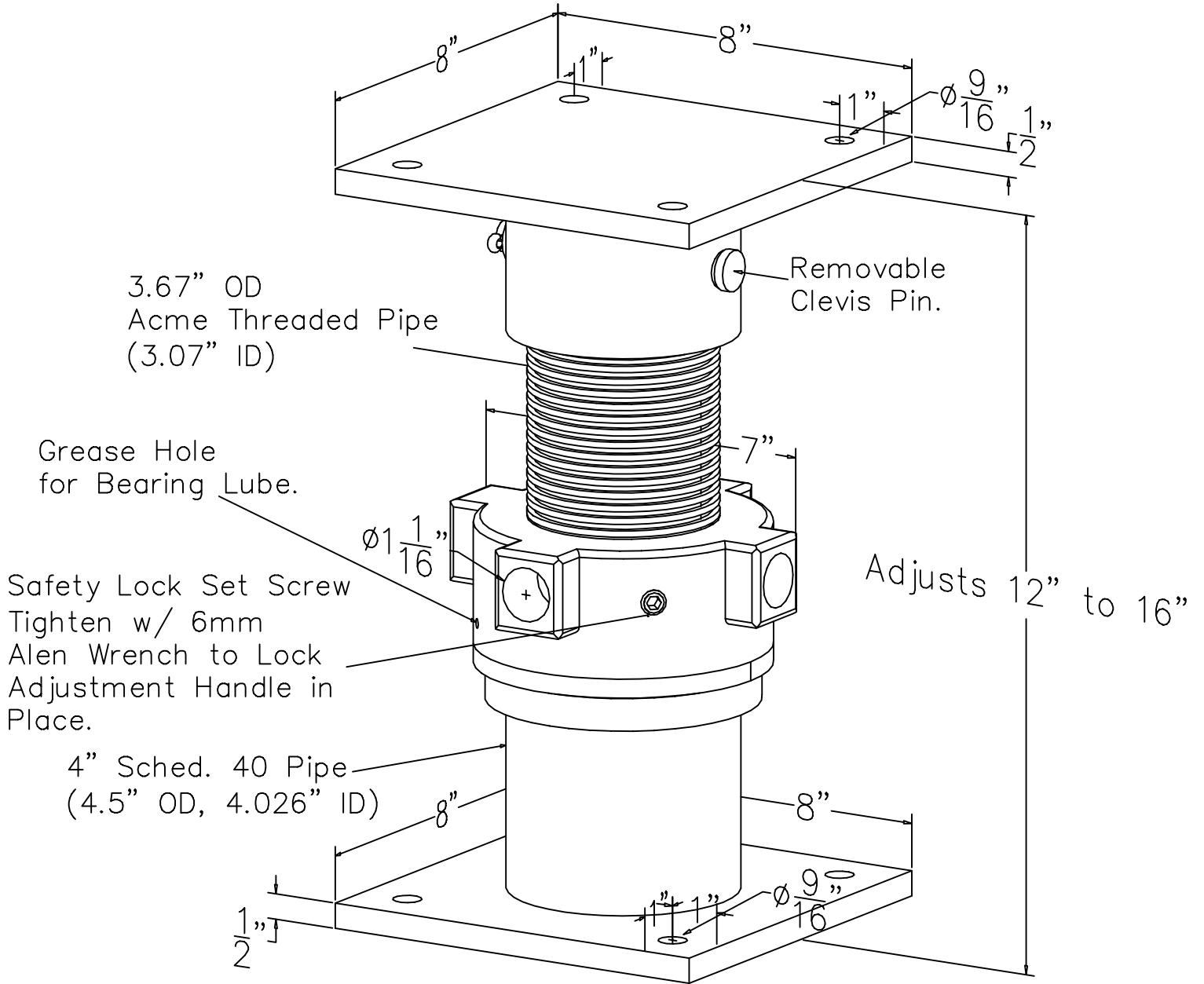
Blg B Ultra Duty Steel Shore BB-12 Adjusts 4" 12" Minimum Height 16" Maximum Height 80,000 Lb. Safe Load Capacity
