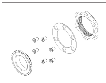
Six-Bolt to CenterLock Adapter
