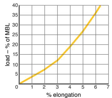
PSR 2000 12 Strand Elongation (%)
