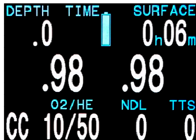
Two sensors can now be used in the external PPO2 monitoring mode (not available on controller models)
