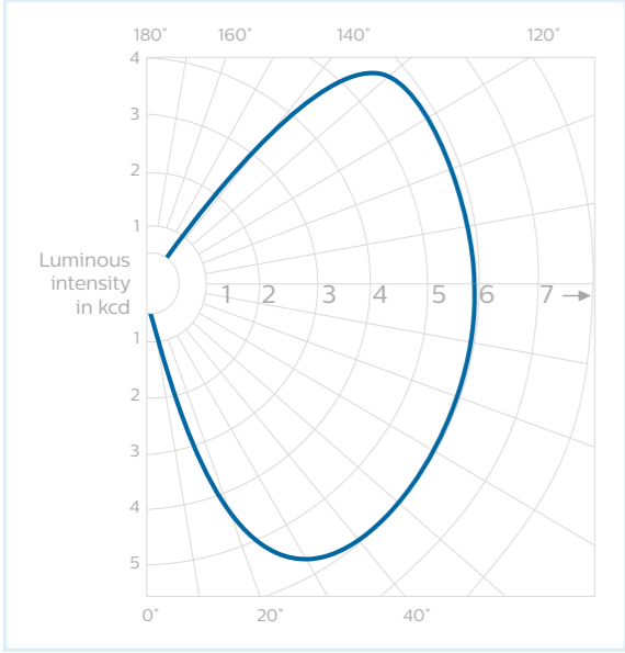
Luminous intensity
