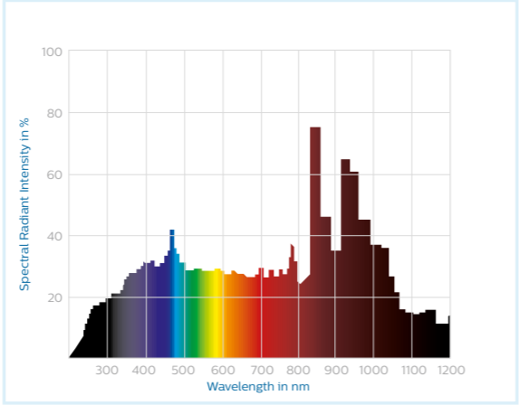
Spectral distribution
