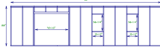
Front Wall Siding Layout (Doors aligned to the left)
