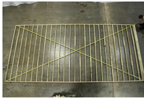
(20) Before proceeding, ensure that floor is square. Both measurements need to be equal.
