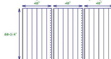
Right Gable Wall Siding Layout
