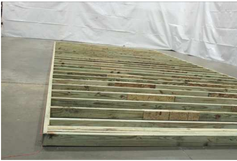
(19) Continue until floor is complete.
