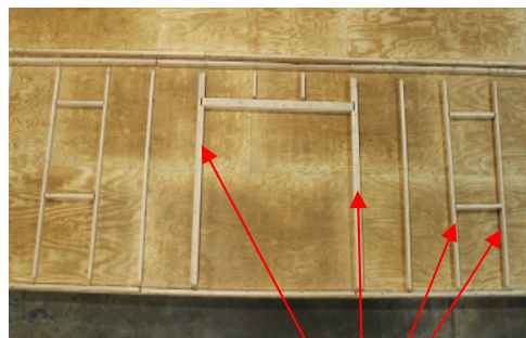
(69) Front wall is done much the same as the back wall except for the door and window studs. Locate double studs with dados for the door, and single studs with dados for the windows.
