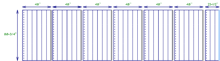
Back Wall Siding Layout
