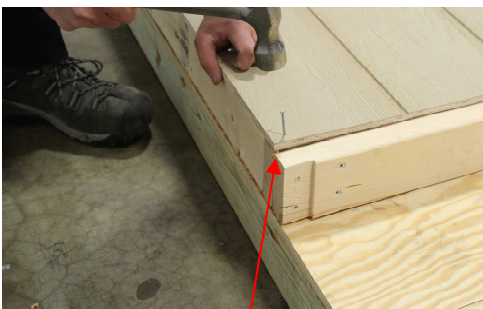
(42) Starting with the left piece, place the siding even with the center of the double top plate, and 1/2" out over the wall stud.
