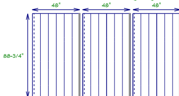
Left Gable Wall Siding Layout
