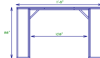
Right Gable Wall Siding Layout
