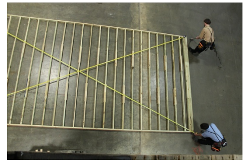
(21) Knock the joists on the end accordingly, till measurements are equal.
