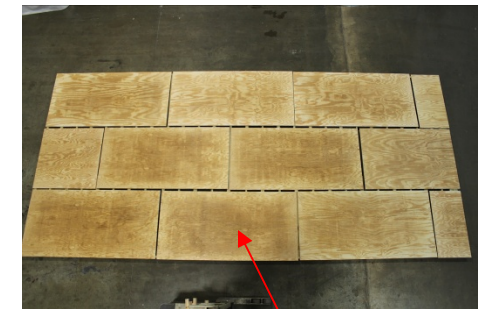
(27) Put the next piece in place, then refer to following step.
