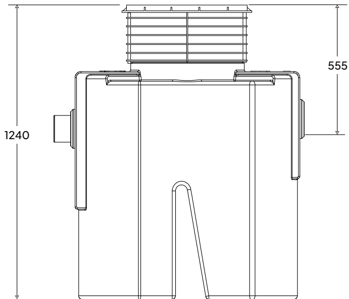
JGTIA – BASE MODEL WITH 500ER EXTENSION RISER FITTED
