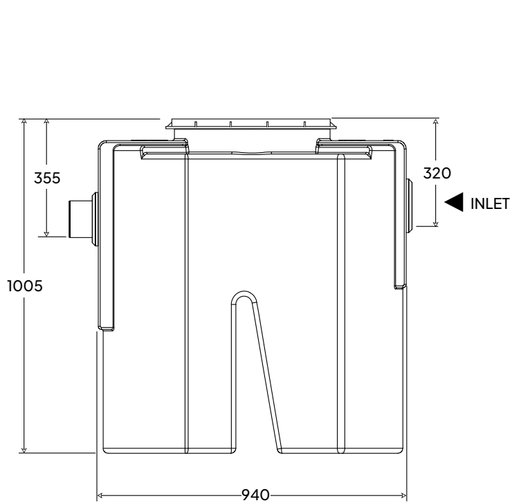
JGTIA – BASE MODEL WITH 500ER EXTENSION RISER FITTED
