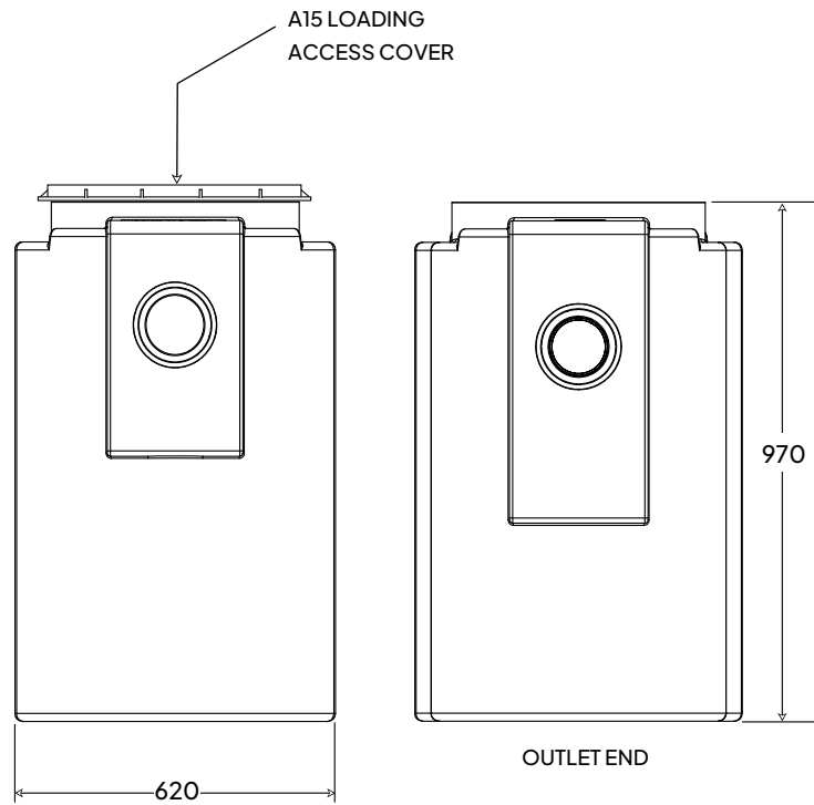
EXTENSION RISER
