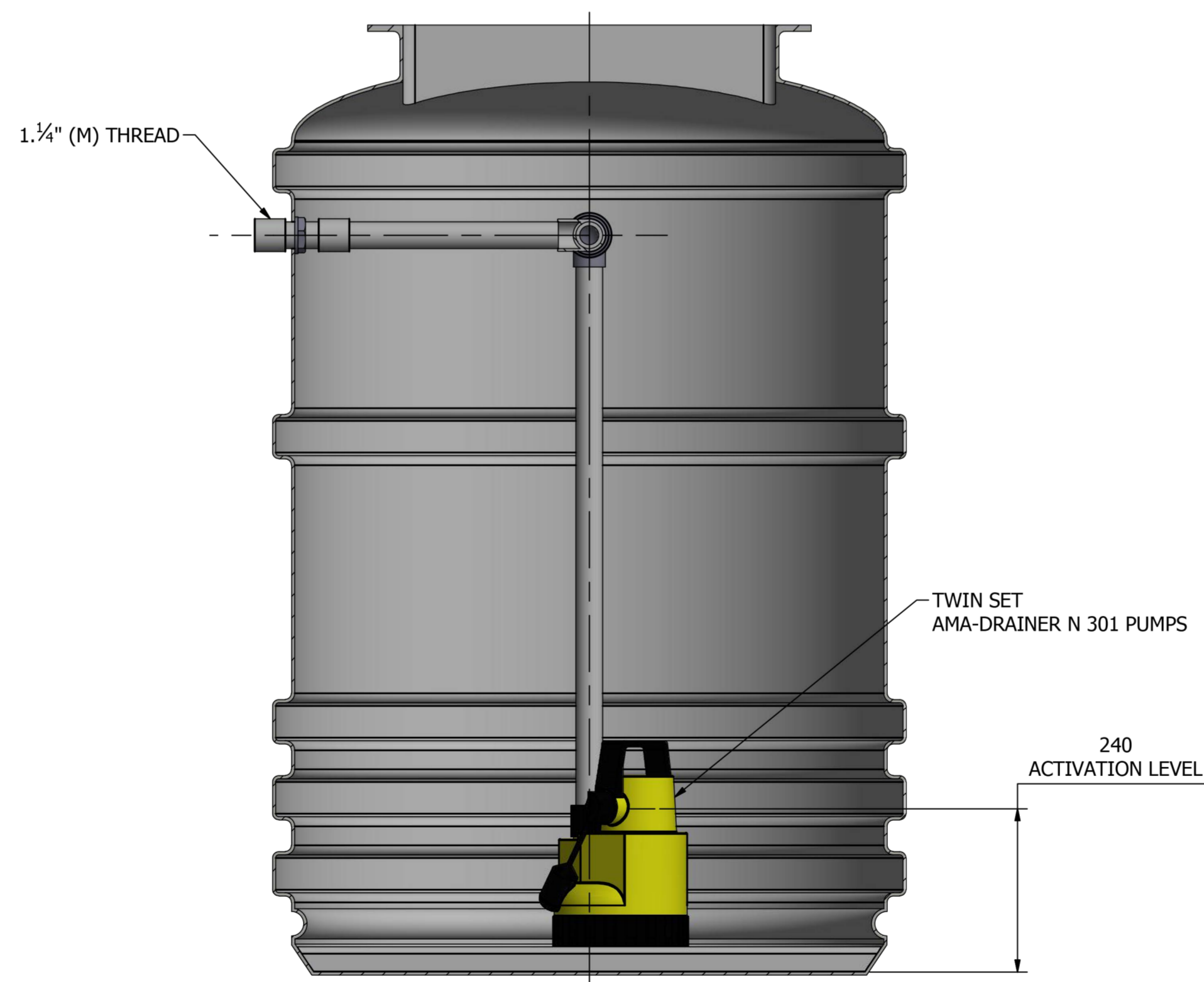
SECTION A-A SCALE 1:7.5
