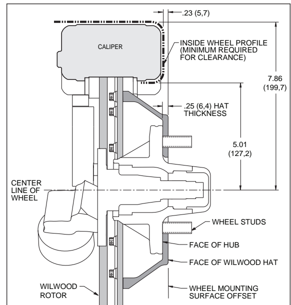
Figure 2. Wheel Clearance Diagram
