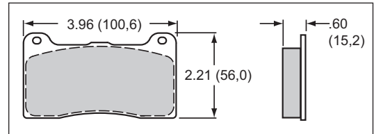
DynaPro Caliper, Type 7816 Pad Dimensions P/N 150-9753K
