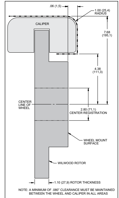
Figure 3B, P/N 140-16131. Wheel Clearance Diagram
