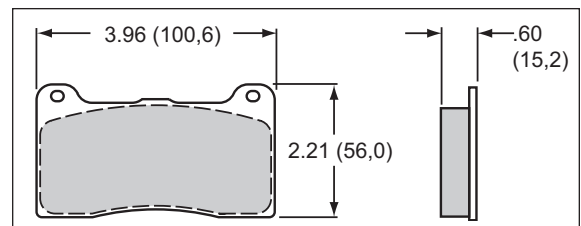
DynaPro Caliper, Type 7816 Pad Dimensions
