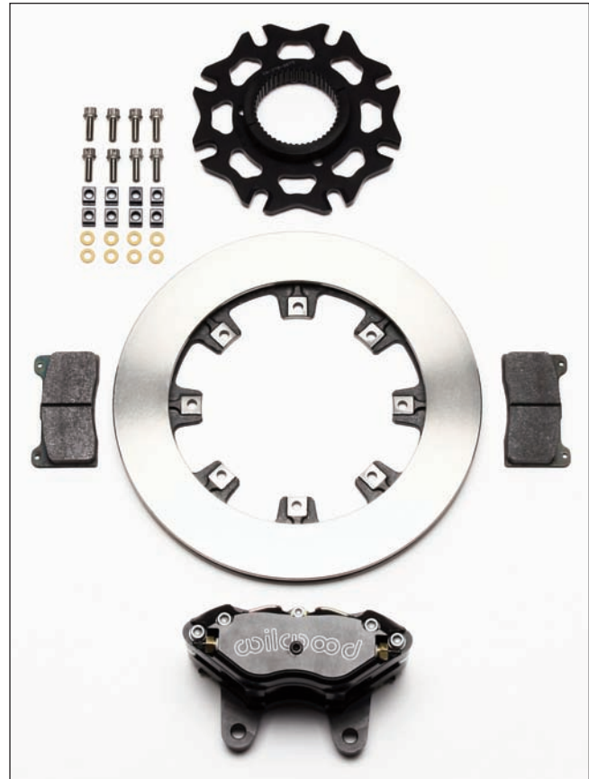
Sprint Narrow DynaPro Inboard Brake Kit Components Kit Part Number 140-10797
