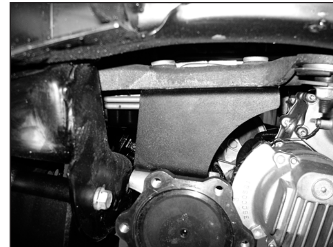
FIGURE 28 - SHOWN WITH DIFFERENTIAL ALREADY INSTALLED
