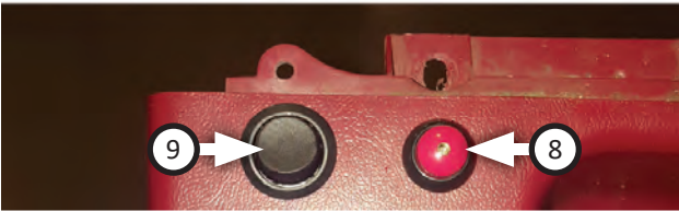
16. Drill and mount On/Off switch (9) and lit momentary switch (8) to console as shown.
