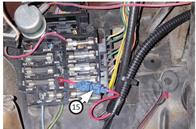
21. Attach red wire to a power source using tap connector (15) if necessary.
