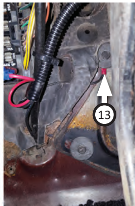
18. Extend momentary switch black ground wire with splice (13) , black wire (5) and eyelet (12) . Ground this wire to chassis (this kit was grounded at firewall).
