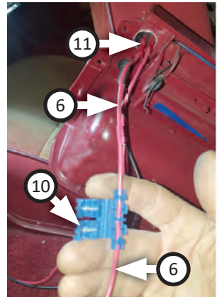
20. Install terminal (11) to red wire (7) then plug it into on/off switch reaming post. Then use fuse holder (10) and more red wire (6) to reach power source.
