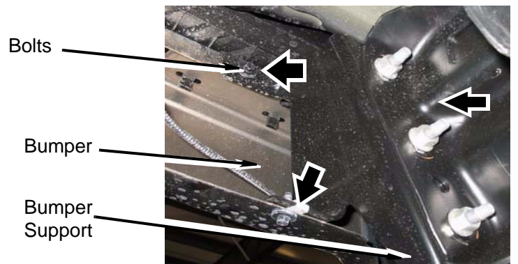
Kit Bolt (3/8"-13 x 1"), Washer (3/8"), Nut (3/8" Nylock)
