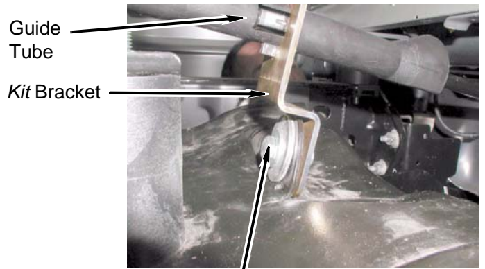
Kit Bolt (3/8"-13 x 1"), Washer (3/8"), Nut (3/8" Nylock)
