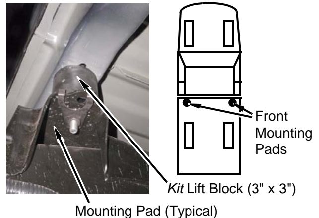
Cab Mounting Locations
