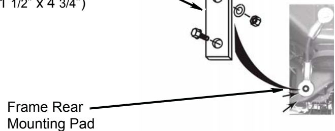
Kit Cab Safety Cable Extension Bracket (1 1/2" x 4 3/4")
