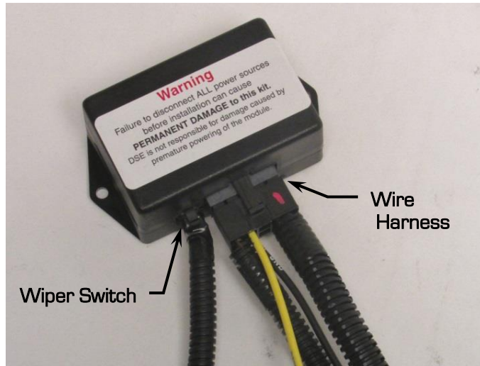
Figure 16 – Connect Wiper Switch & Harness to Module
