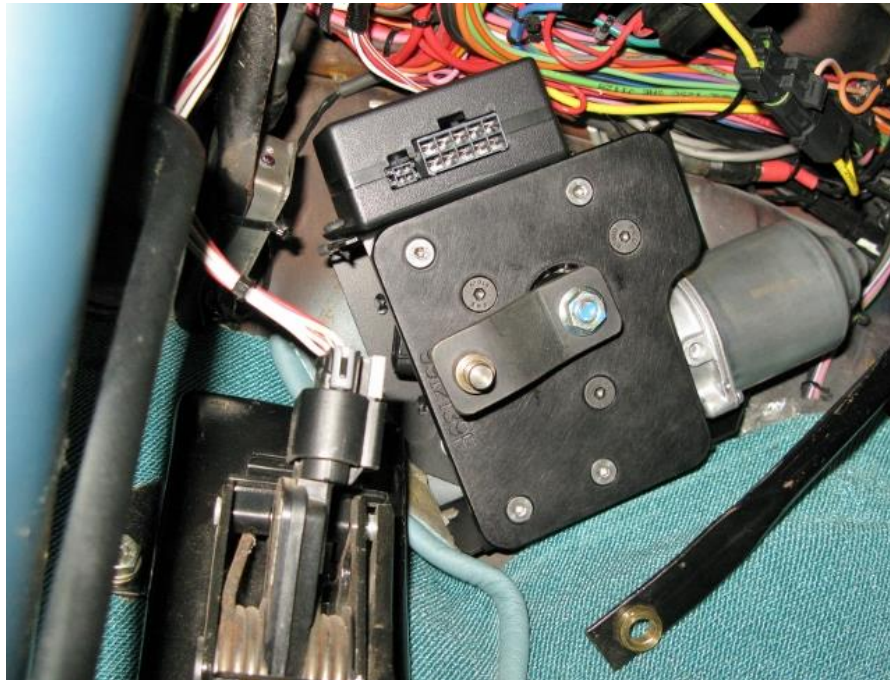
Figure 6 - Install Wiper Motor & Adapter Plate
