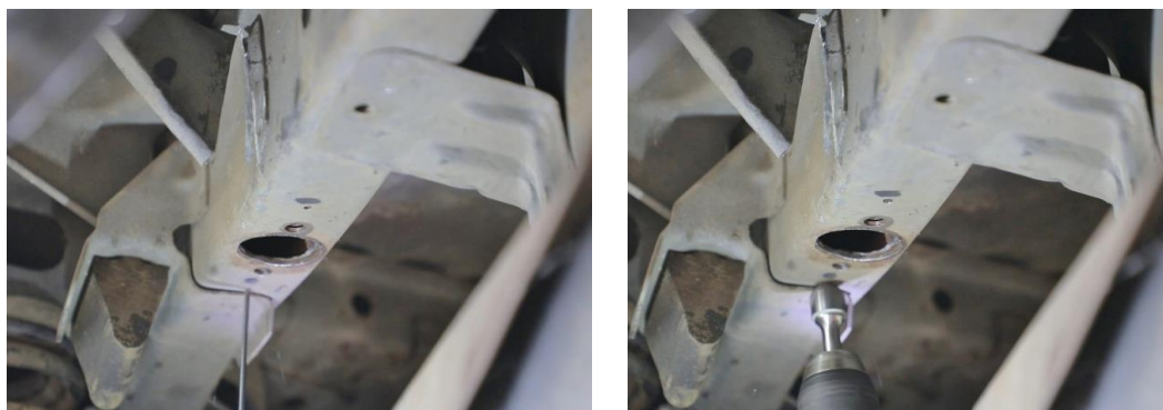
Figure 29 - Drill & Chamfer Nut Plate Mounting Holes
