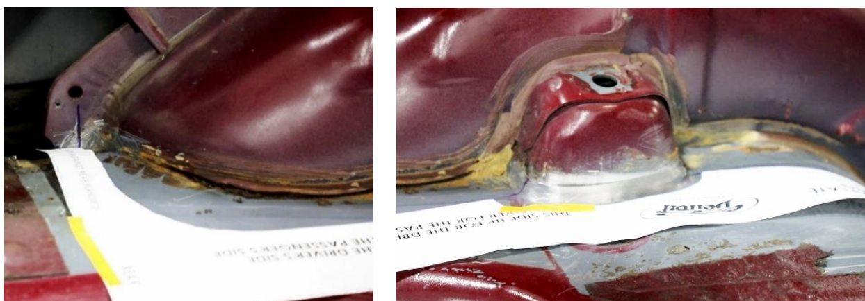
Figure 14 - Locate Rear Template
