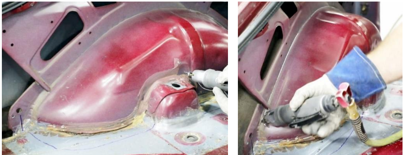
Figure 17 – Cutout Inner Wheel Tub
