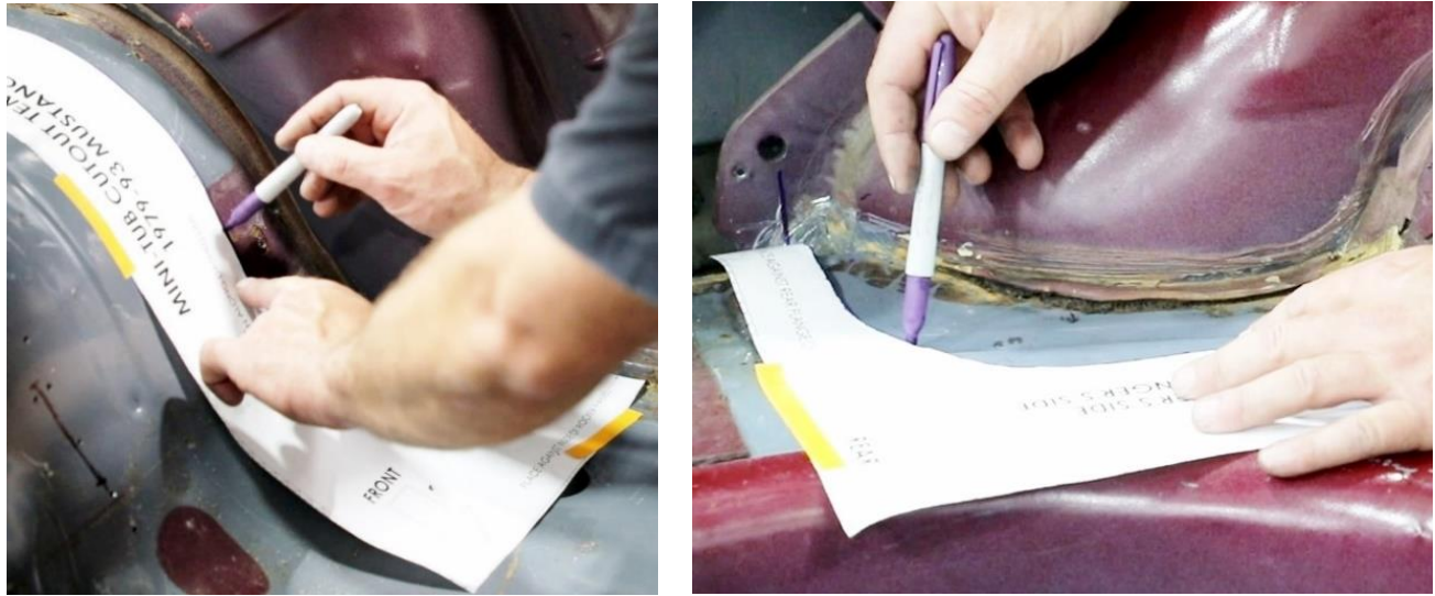
Figure 16 – Draw Cut Line
