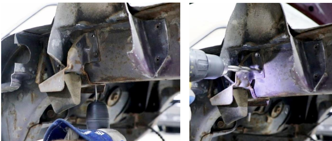
Figure 23 - Drill out Spot Welds
