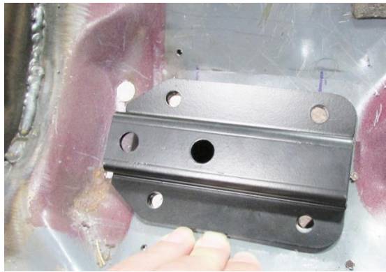
Figure 47 - Drill Bracket Mounting Holes
