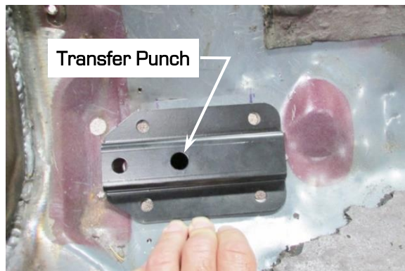
Figure 48 - Transfer Punch
