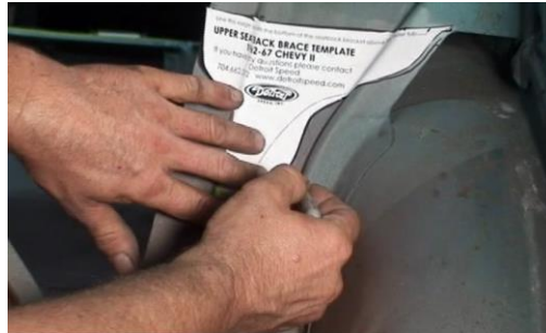
Figure 4 - Tracing the Template on the Seatback Brace (62-65 model shown)
