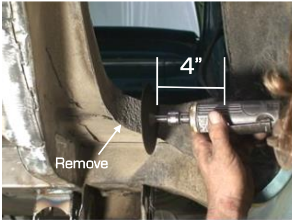
Figure 8a - Cutting the Factory Flange
