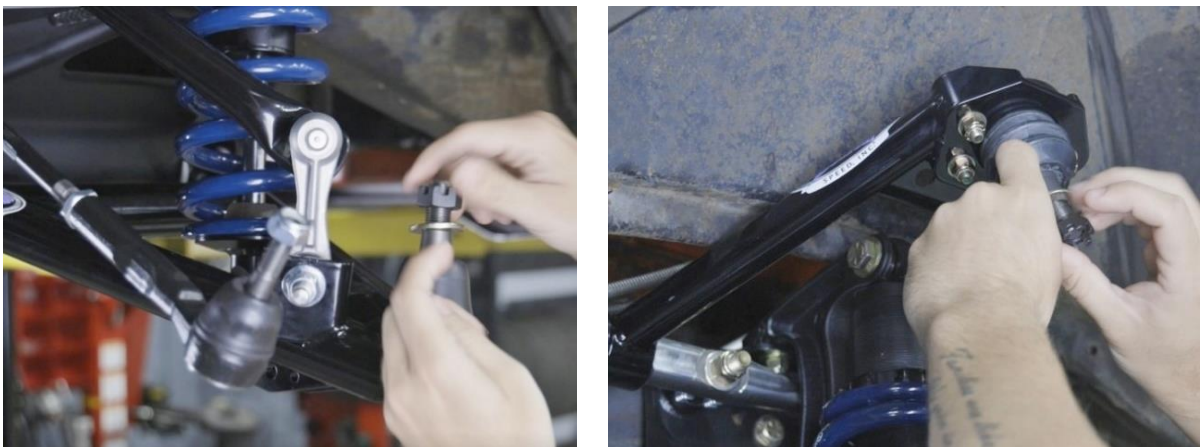
Figure 92 - Remove Ball Joint Hardware
