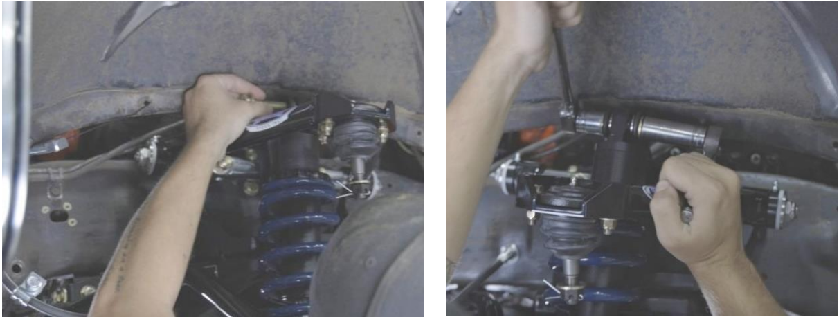
Figure 82 – Install Upper Shock Mounting Hardware
