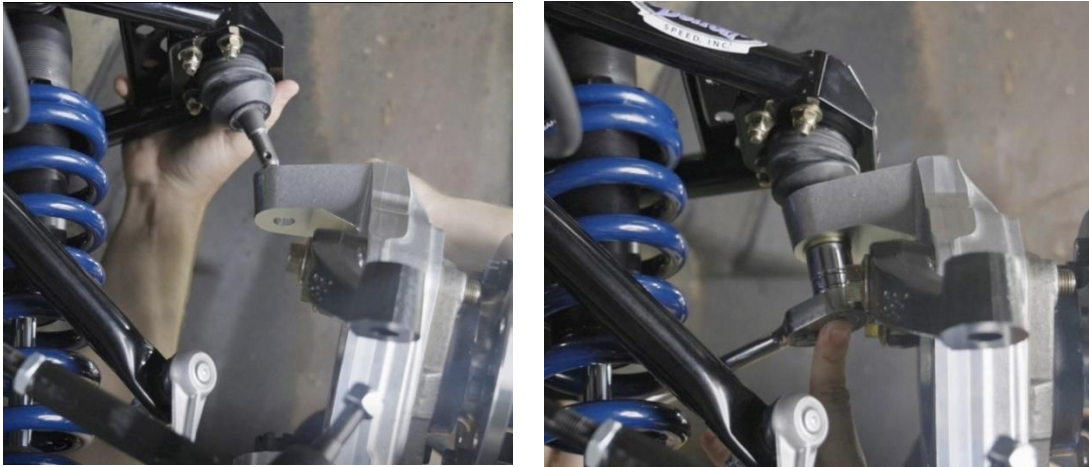
Figure 94 - Install Upper Ball Joint
