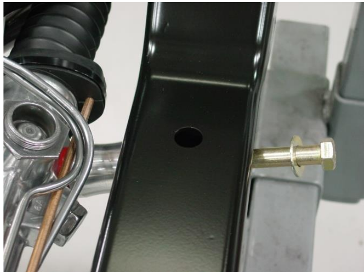
Figure 15 – Attaching the Rack to the Cross Member
