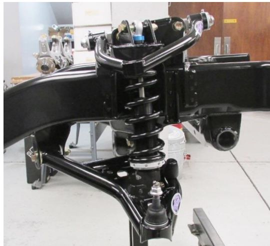
Figure 12 - Installed Coilover View (Passenger Side)
