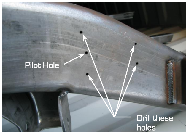
Figure 2 - Locating the Holes to be Drilled
