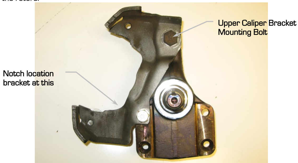
Figure 3 - Notching Stock Caliper Bracket
