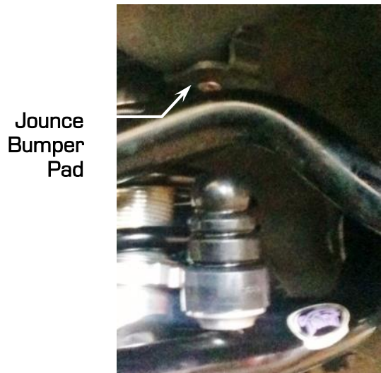
Figure 1 - Jounce Bumper Pad
