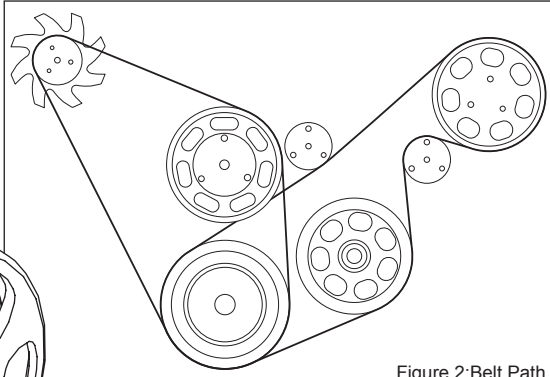
Figure 2: Belt Path
