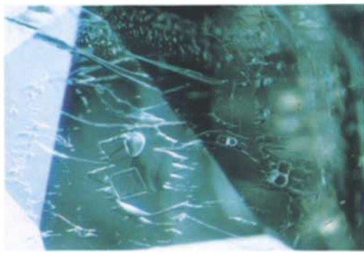
Fig. 8. Primary axial healing fissure with flat cavities containing different exsolution components of constant volume proportions of s/l/g. Largest gas bubble with a delicate crescent seam of liquid carbon dioxide (CO 2 ), largest daughter crystal with a rhombohedral habit and zonal structure (a carbonate), smaller daughter crystals with a cubic habit (halite). Long diagonal of the rhombohedron circa 0.25 mm.
