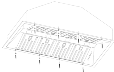
FRHRE5337-60: 8 screws
