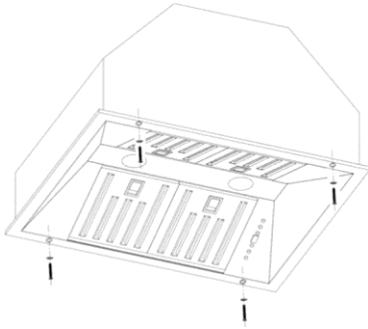
FRHRE5337-30: 4 screws.
