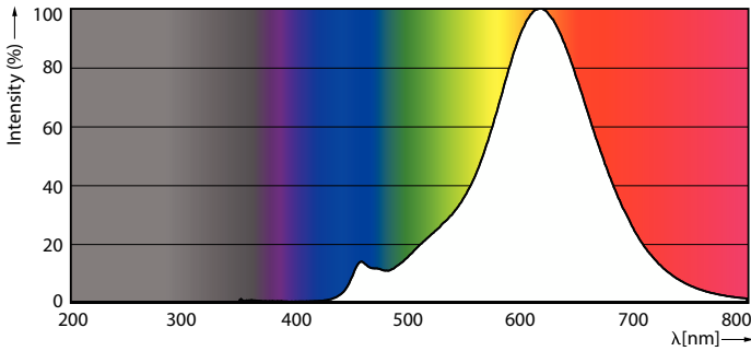
Spectral Power Distribution Colour - 4.5A19/VIN/820/E26/CL/GL/DIM 4/FBH T20
