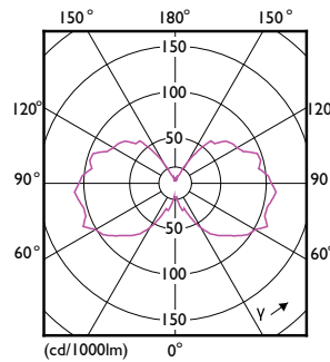
Light Distribution Diagram - 4.5A19/VIN/820/E26/CL/GL/DIM 4/FBH T20
