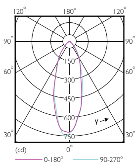
Light Distribution Diagram - LEDspot GU10 6-50W D 830 35D 120V PF
