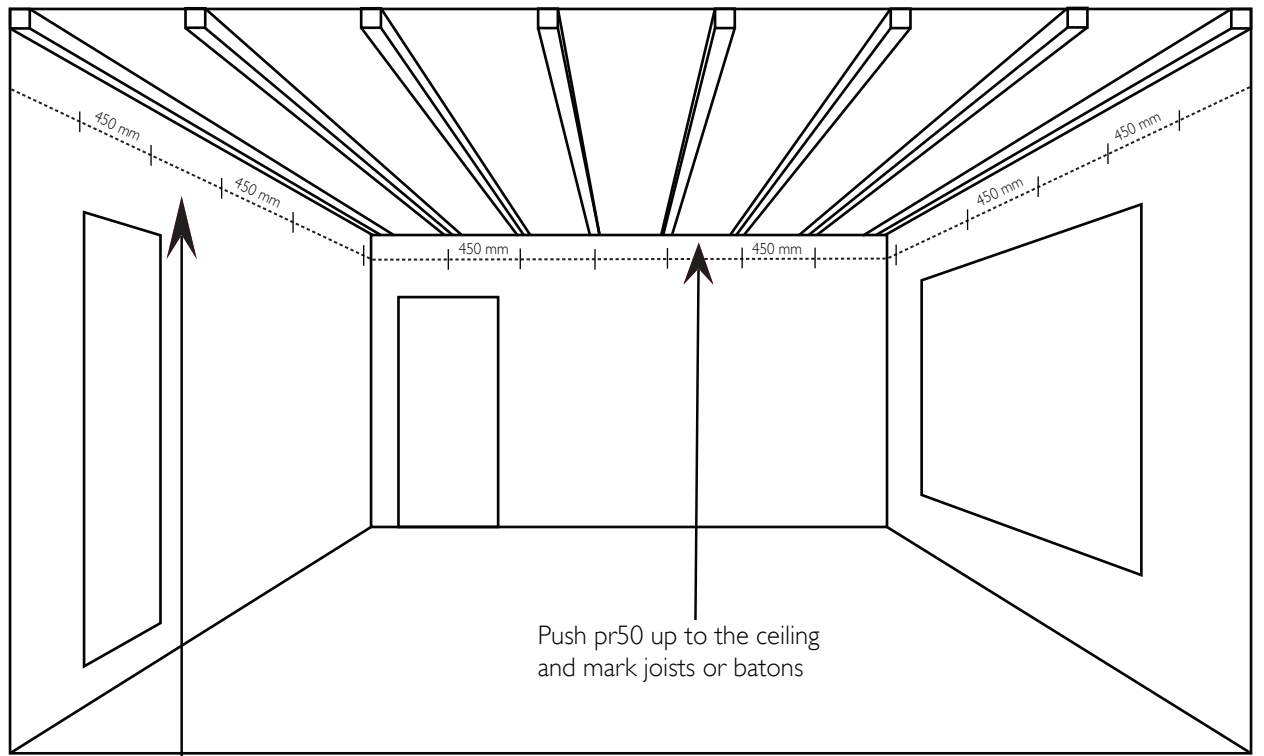
Fix pr50 at 450mm centre
