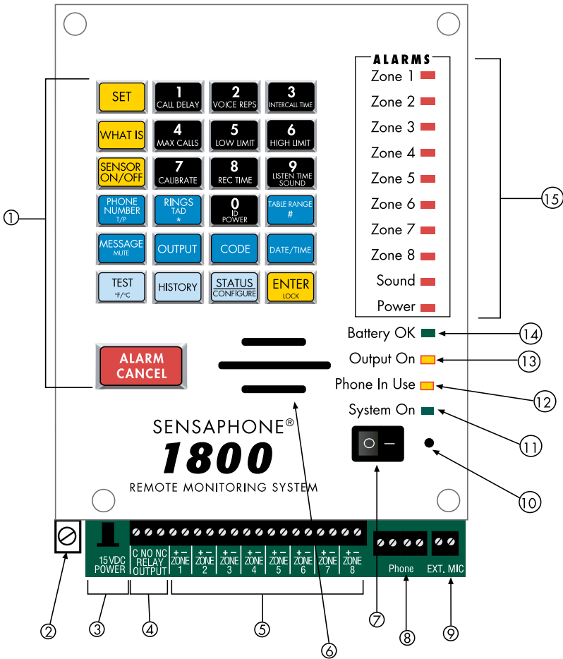
Figure 1: Sensaphone 1800 diagram
